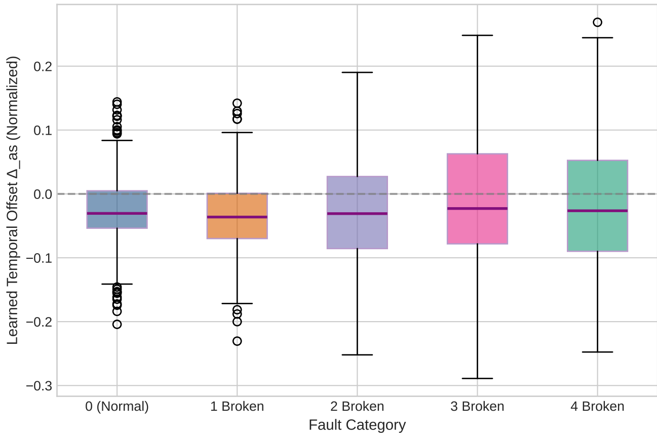
Learned Inter-Modality Lag Distribution by Fault Class ( \Delta_{as} )
